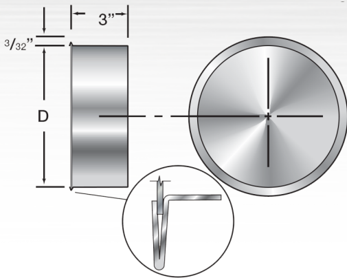
Plugs & Caps
