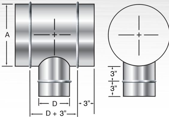
Plain Tee
