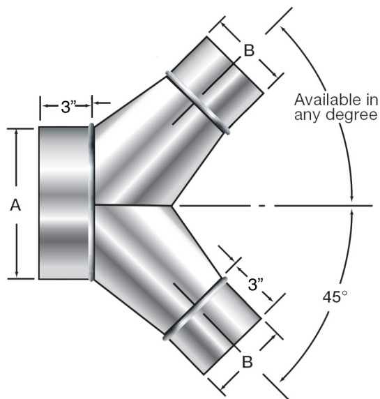
Y Branch or Pant Wye
