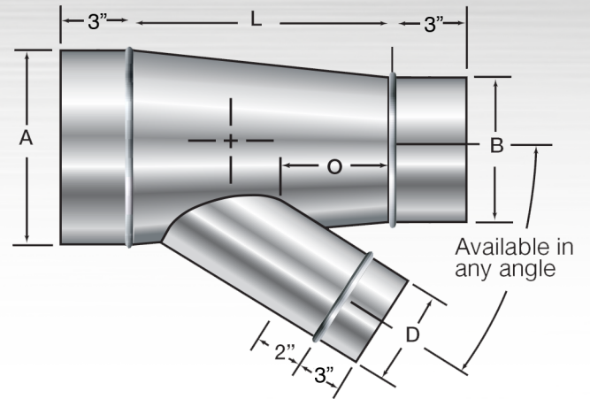
Tapered Reducing Lateral (Standard)
