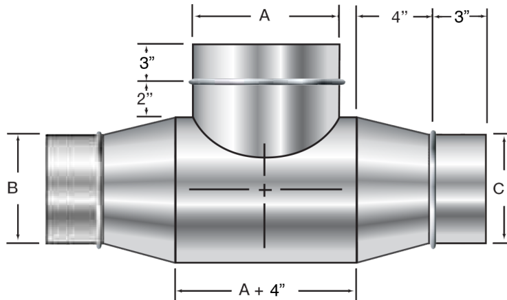
Bullhead Tee
