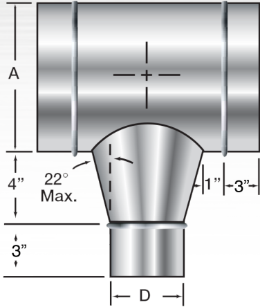
Conical Tee
