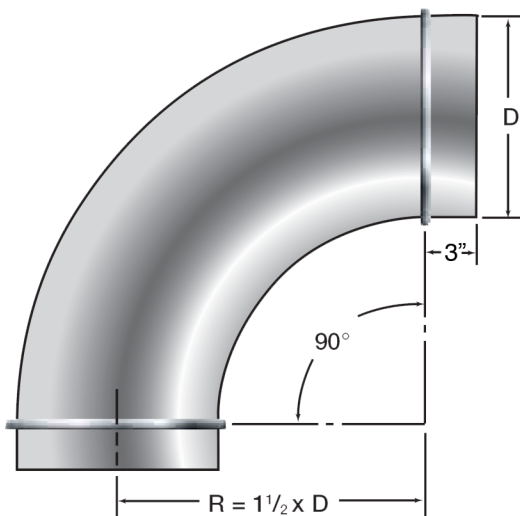
90° Die-Formed Elbow
