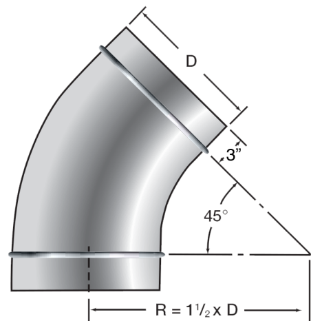
45° Die-Formed Elbow
