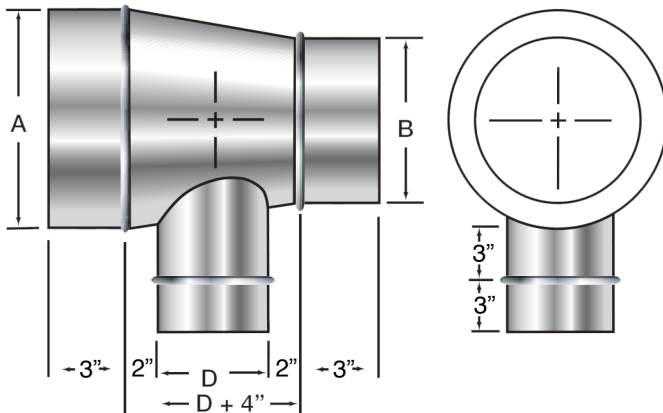
Reducing Tee
