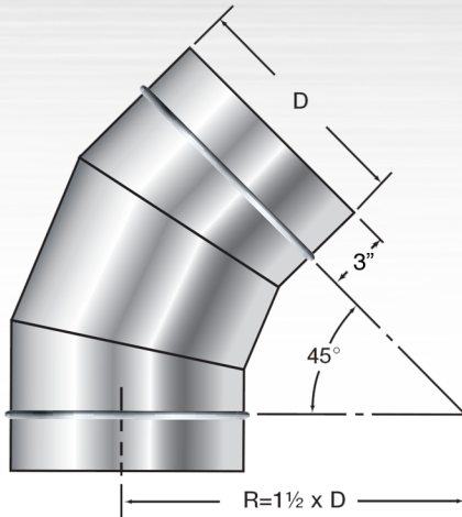
45° Gored Elbow
