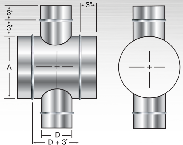
180° Cross Tee
