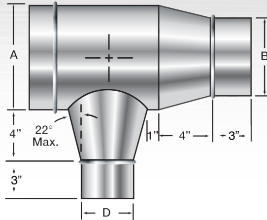
Conical Reducing Tee
