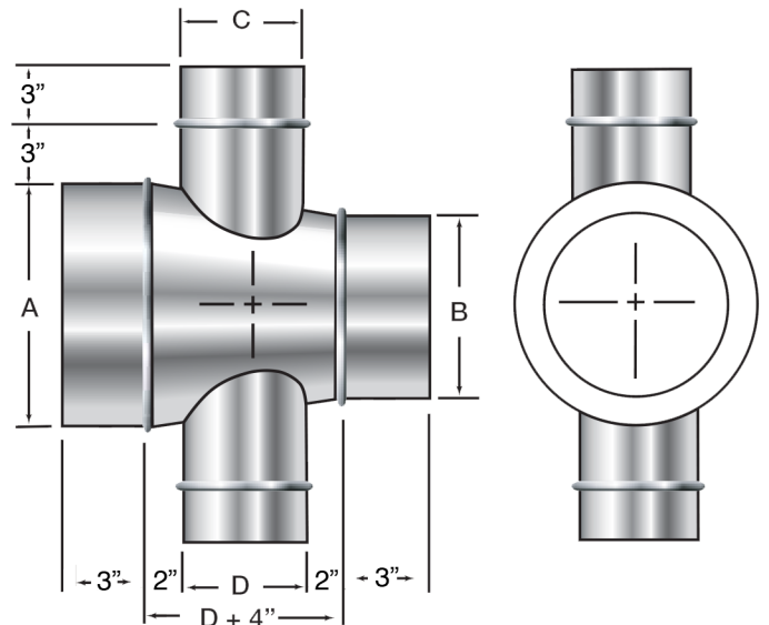
180° Reducing Cross
