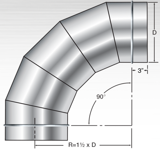
90° Gored Elbow
