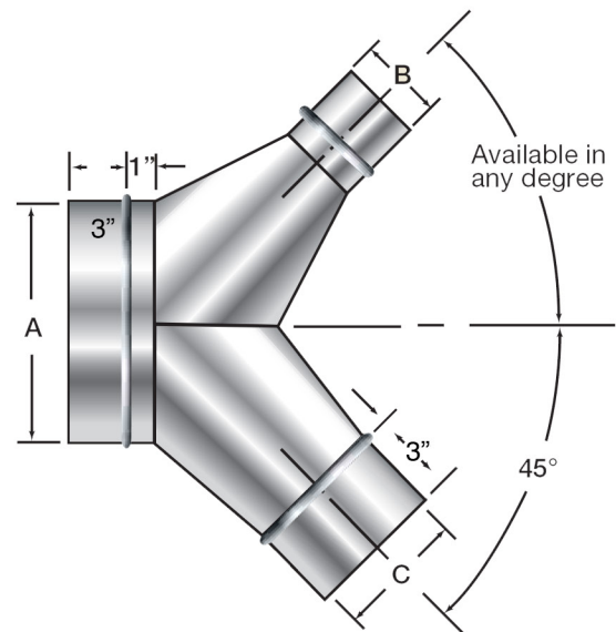
Reducing Y Branch
